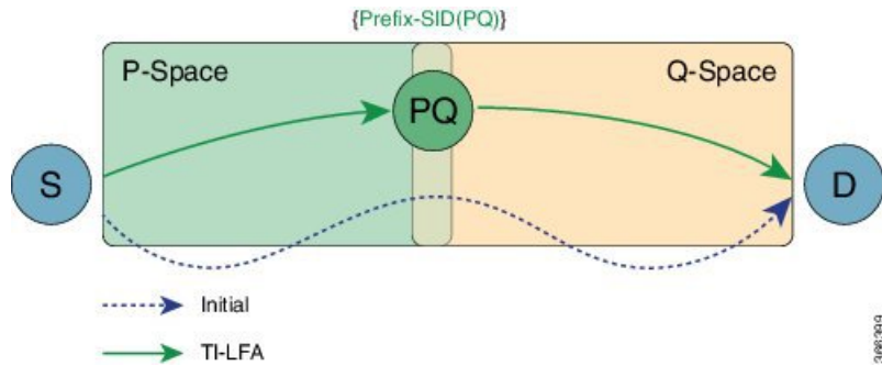
Figure 3: TI-LFA: { Prefix-SID(PQ) }
