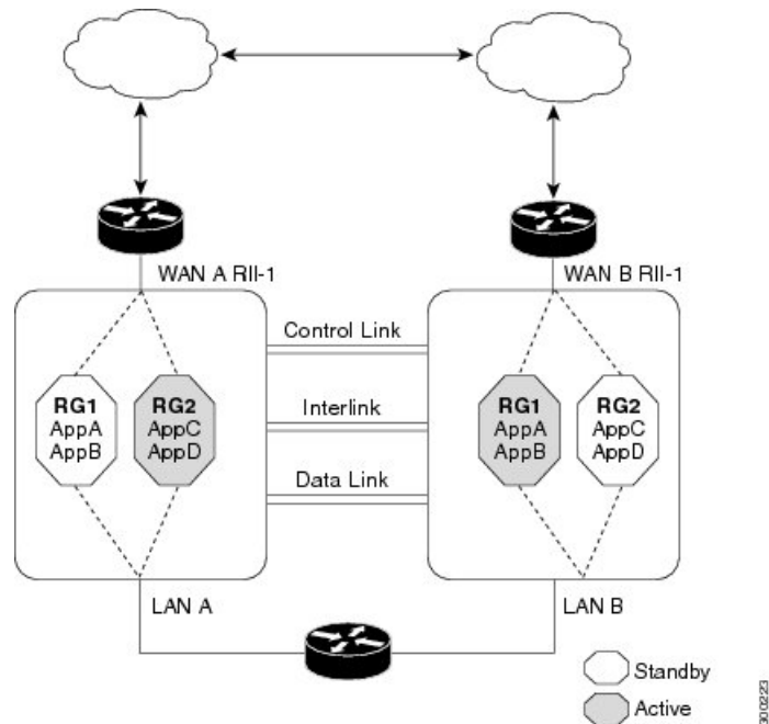
Figure 1: Asymmetric Routing Scenario
