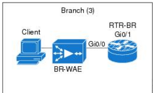
Figure 6 WAAS Inline Path Branch Deployment
