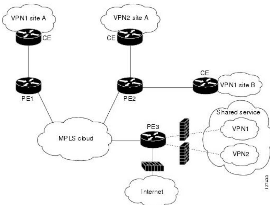
Figure 14 Hub-and-Spoke Network
