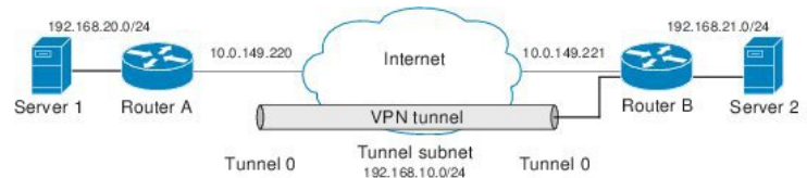
Figure 3: IPsec Configuratoin
