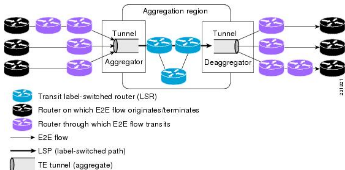
Figure 1: TBAC Overview
