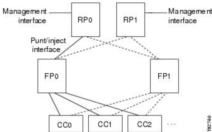
Figure 1: Abstract Illustration of a Cisco ASR 1000 Series Router with Dual RPs and Dual Forwarding Panes
