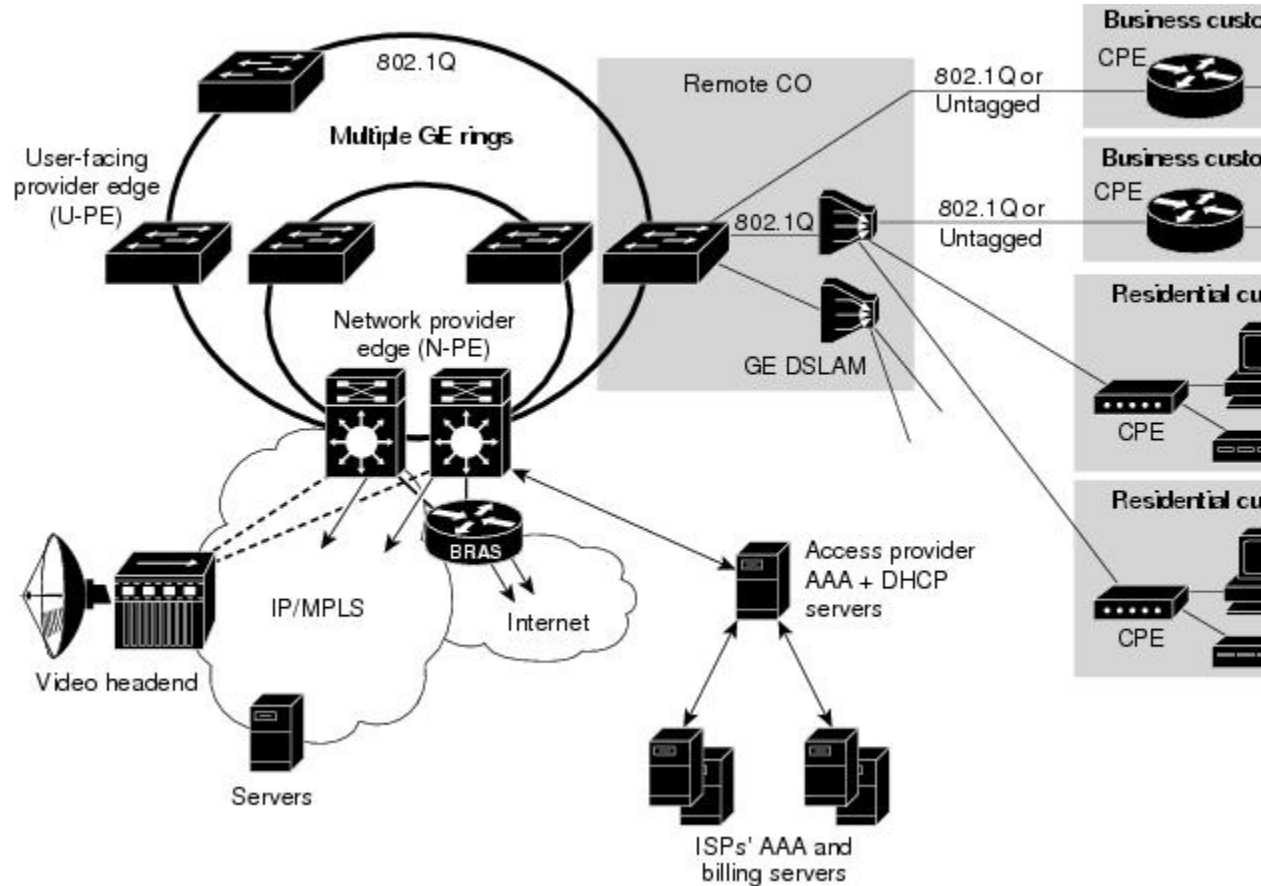
Figure 1 Ethernet DSL Access Network
