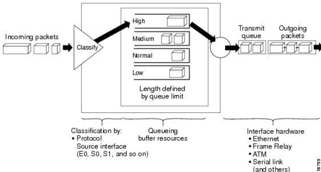
Figure 3 Priority Queueing
