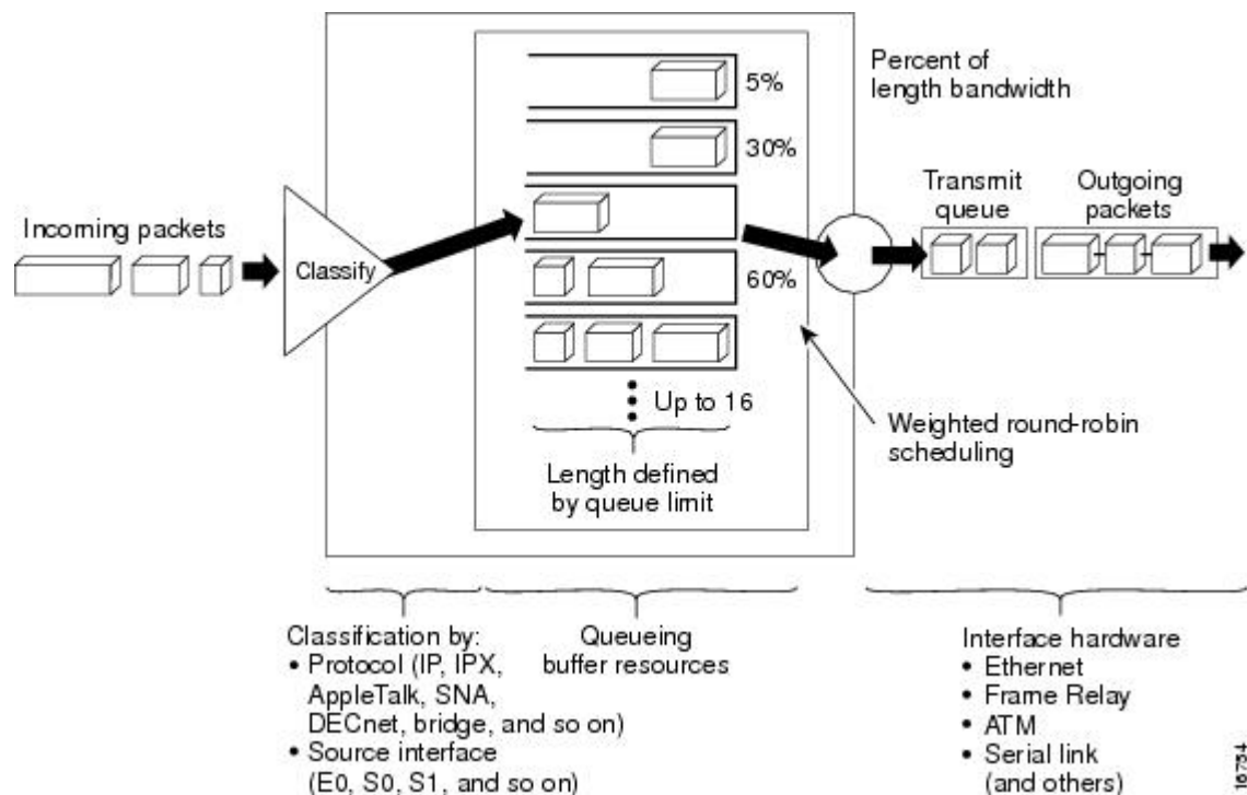
Figure 2 Custom Queuing
