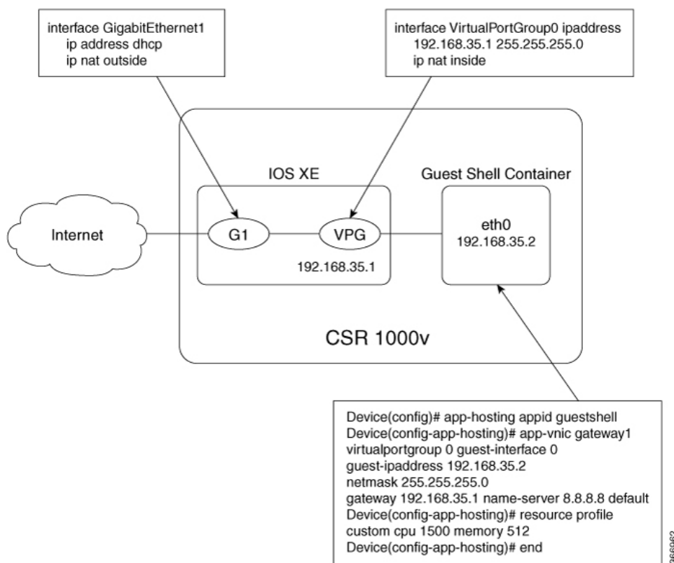
Figure 3: Managing the Guest Shell using Application Hosting
