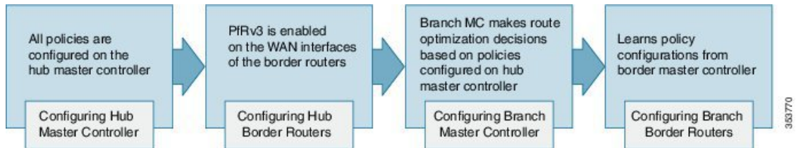
Figure 2: PfRv3 Workflow
