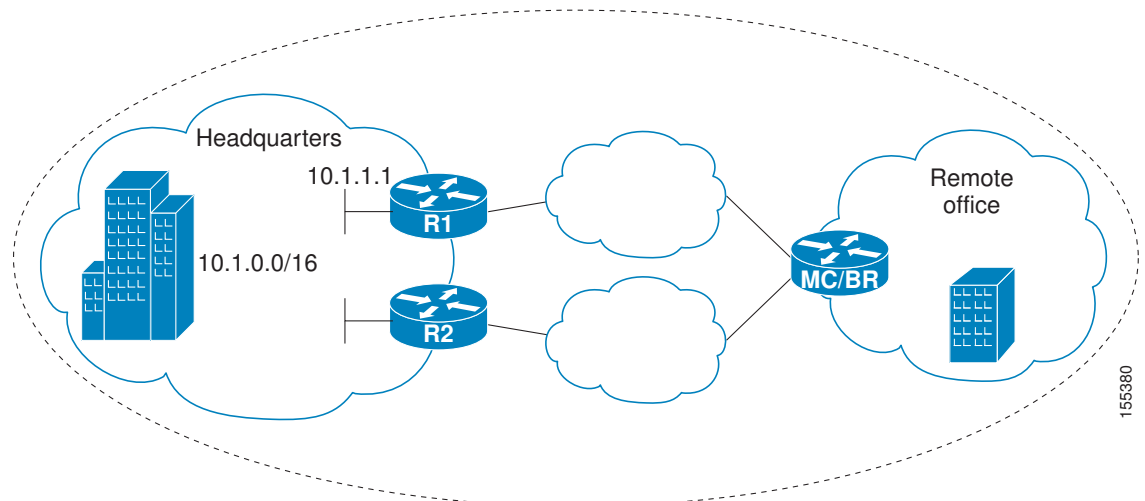
Figure 6 OER Network Topology Optimizing Voice Traffic Using Active Probes
