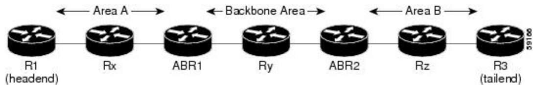
Figure 1: Multiarea Network
