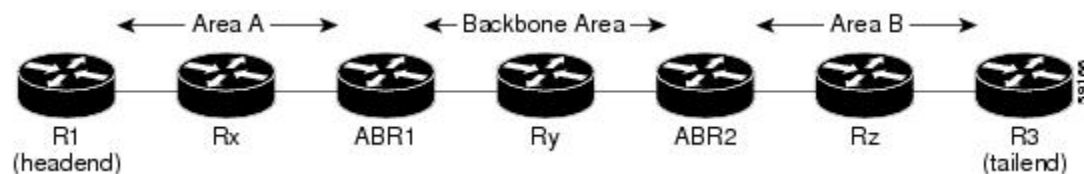
Figure 1 Multiarea Network
