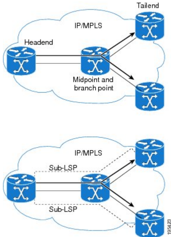
Figure 1 Basic P2MP TE Tunnels
