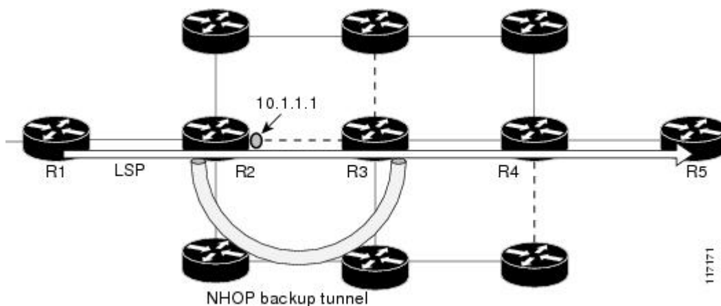
Figure 3 NHOP Backup Tunnel
