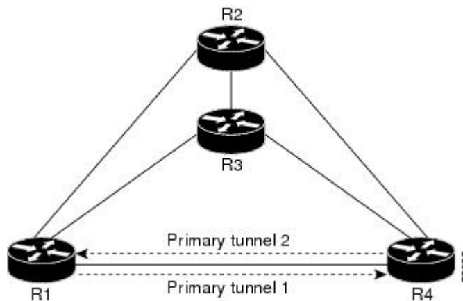
Figure 5: Overloaded Link
