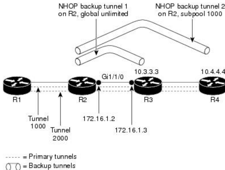
Figure 2: Backup Tunnels
