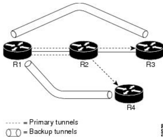
Figure 2: Backup Tunnels that Terminate at Different Destinations
