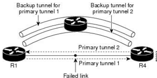
Figure 3: Backup Tunnels Share a Link
