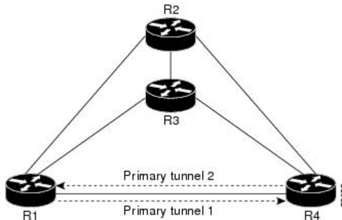
Figure 4: Overloaded Link
