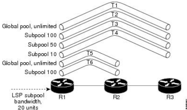
Figure 5: Choosing from Among Multiple Backup Tunnels
