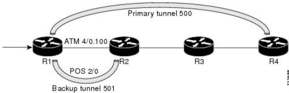
Figure 6: Protected LSPs
