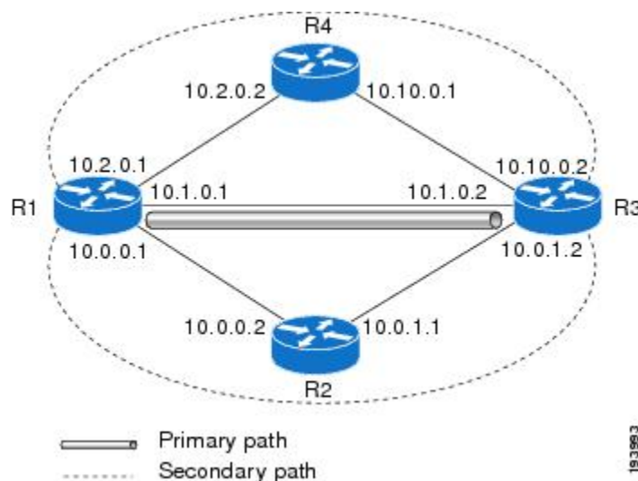
p Network Topology for Enhanced Path Protection
