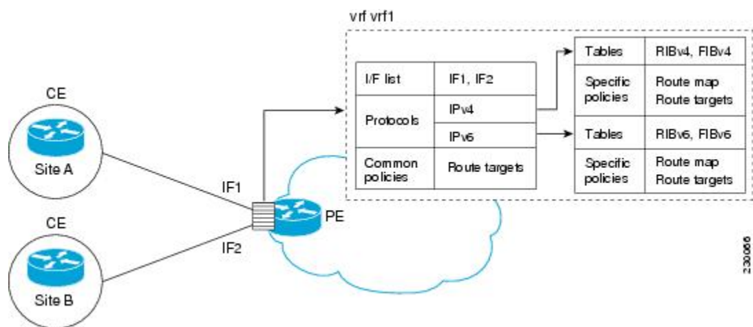
Figure 2: Multiprotocol VRF
