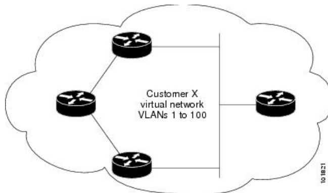
Figure 11: Layer 2 Network Topology without Proper Convergence
