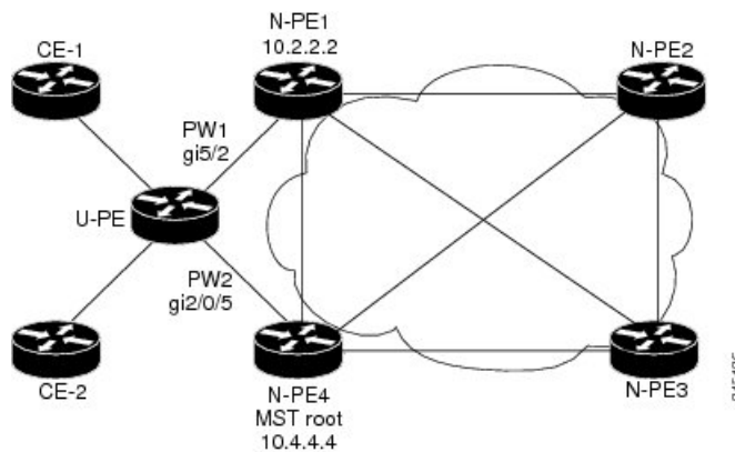
Figure 15: H-VPLS N-PE Redundancy with MPLS Access Topology
