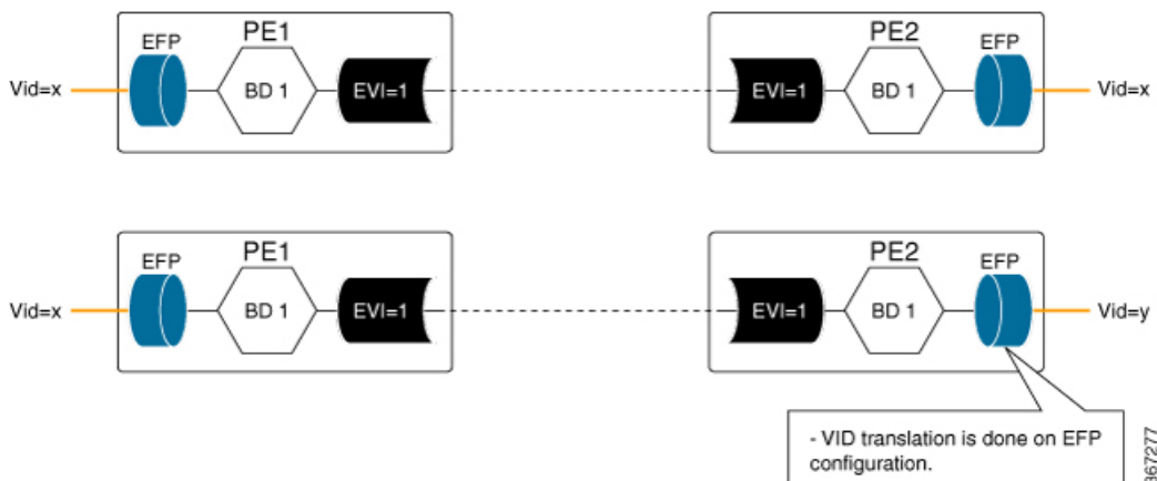
Figure 18: VLAN-Based Service Interface
