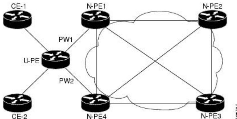
Figure 14: H-VPLS N-PE Redundancy for MPLS Access Based on Pseudowire Redundancy
