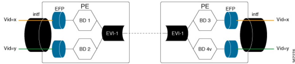
Figure 20: VLAN-Aware Bundle Service Interface
