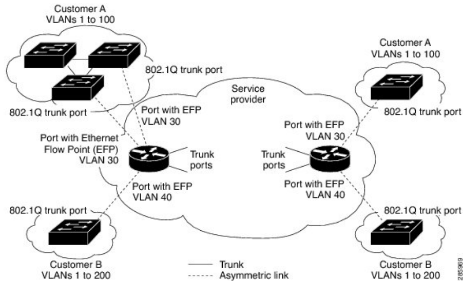
Figure 11: Layer 2 Network Topology without Proper Convergence
