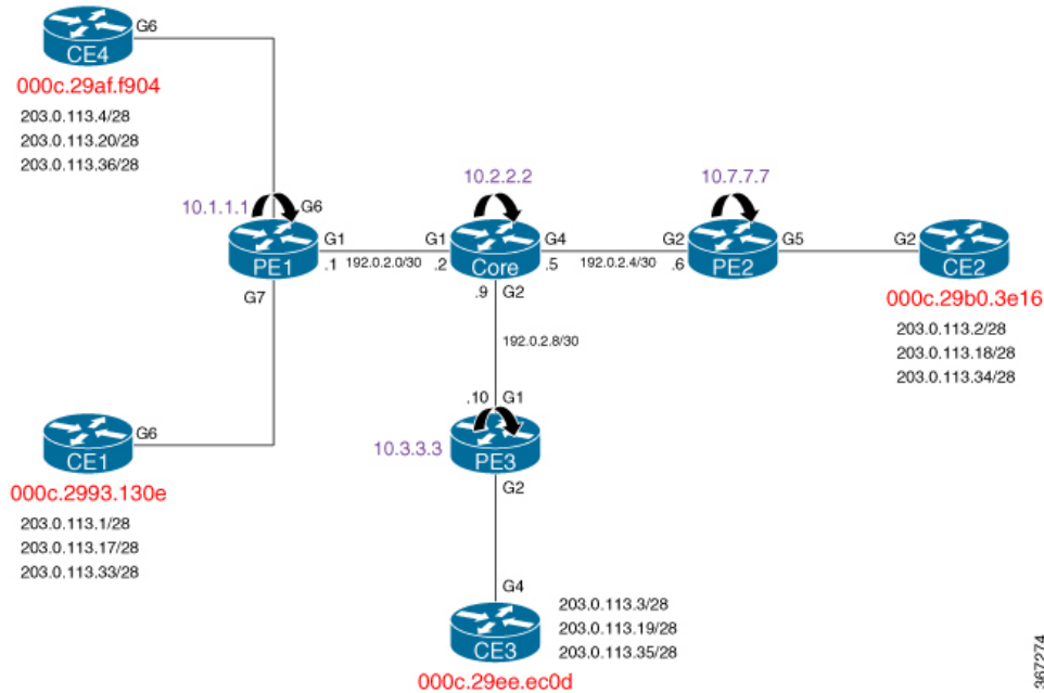
Figure 21: EVPN Single Homing
