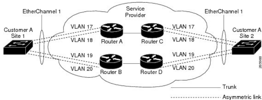
Figure 12: Layer 2 Protocol Tunneling for EtherChannels
