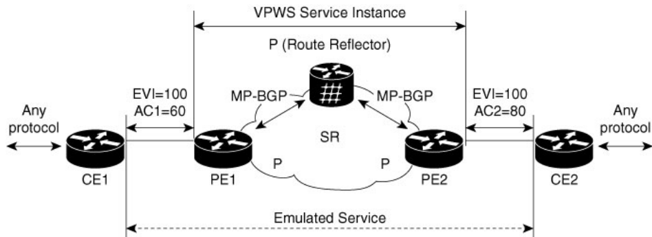
Figure 13: EVPN-VPWS over SR Configuration
