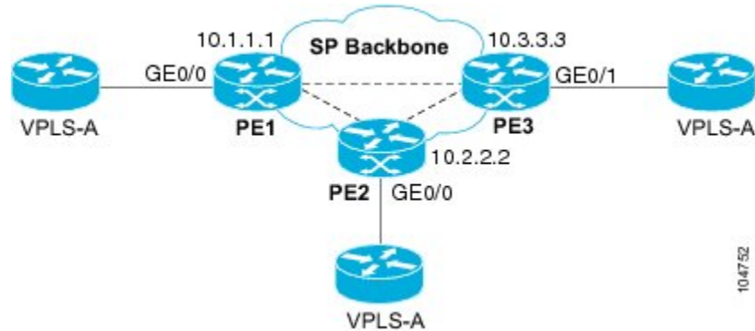
Figure 3: VPLS Configuration Example
