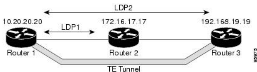
Figure 2 MPLS LDP: NSF/SSO Support and Graceful Restart Configuration Example
