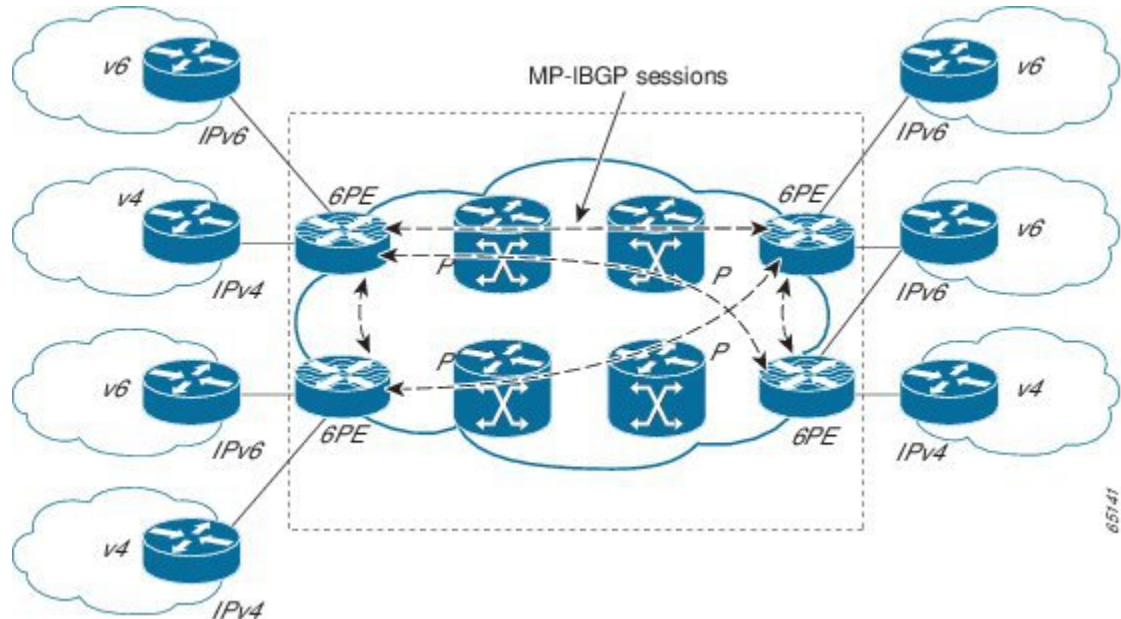
Figure 1: 6PE Device Topology
