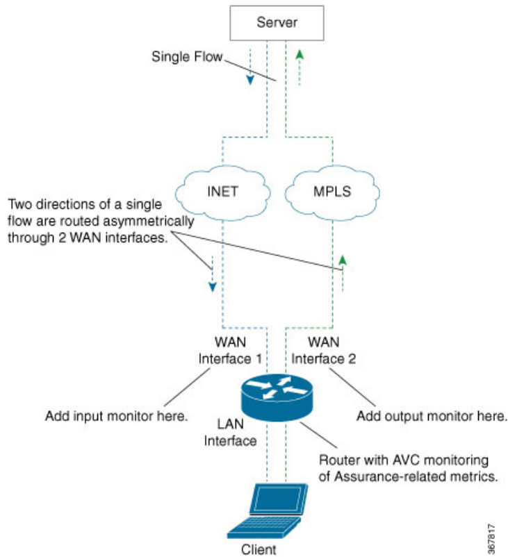
Figure 2: Asymmetric Routing
