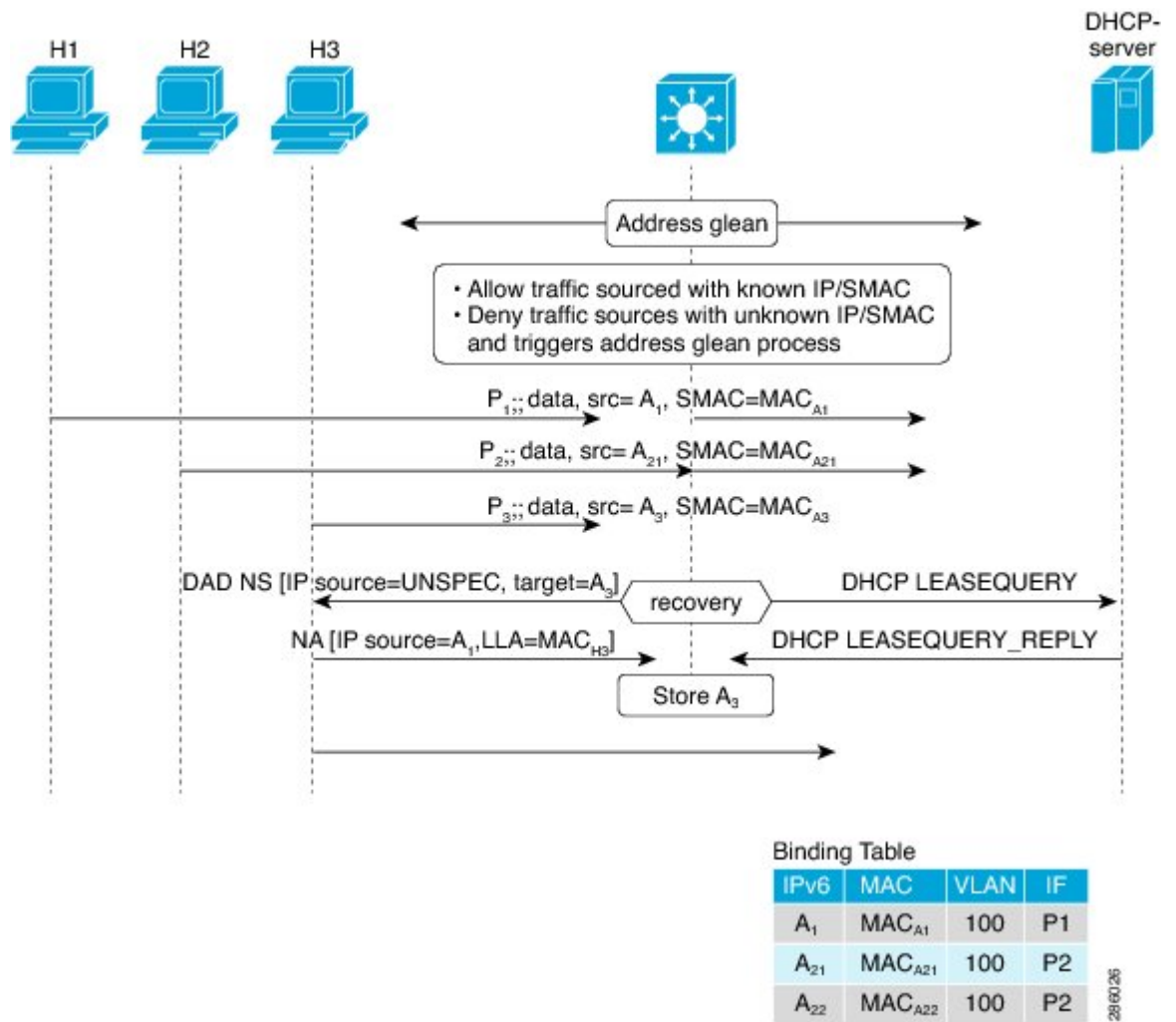
Figure 2: IPv6 Source Guard and Address Glean Overview
