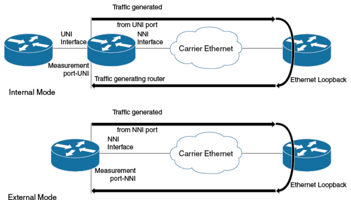
Figure 1: Traffic Generator Topology
