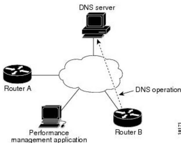
Figure 1: DNS Operation
