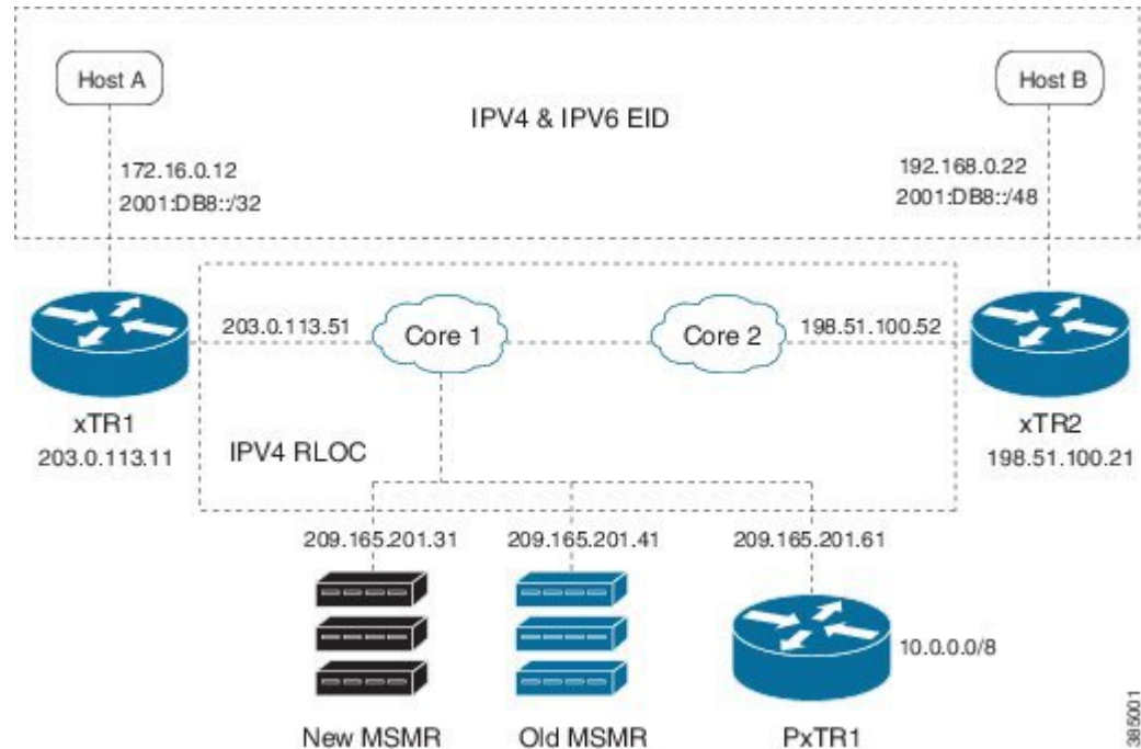
Figure 2: LISP Reliable Registration Topology
