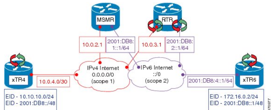
Figure 1: LISP - Disjoint RLOC Domains Topology
