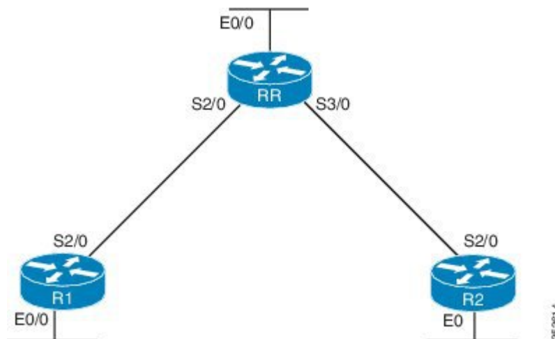
Figure 1: BGP Route Reflector Topology
