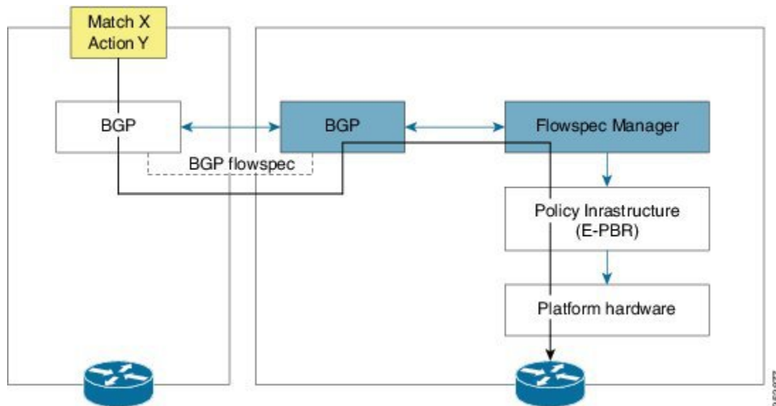
Figure 1: BGP Flow Specification Model
