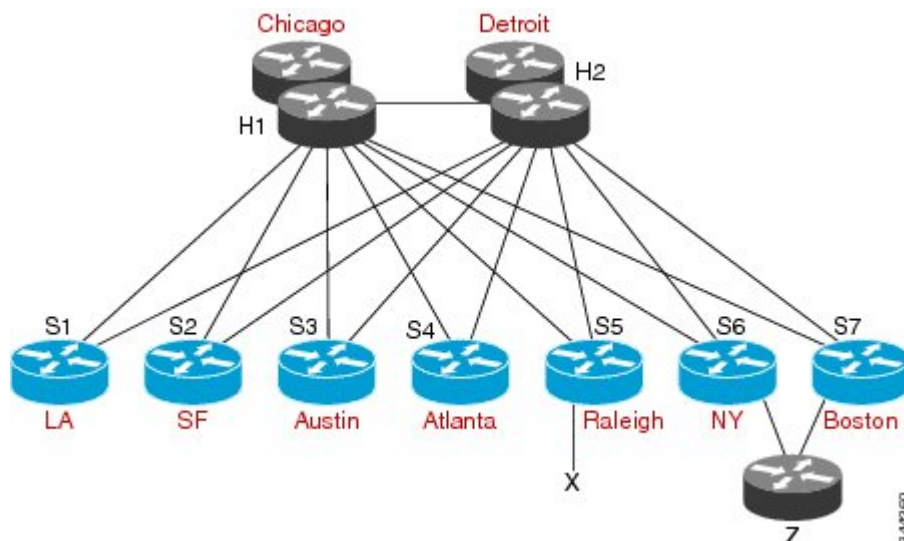
Figure 3: DMVPN Deployment
