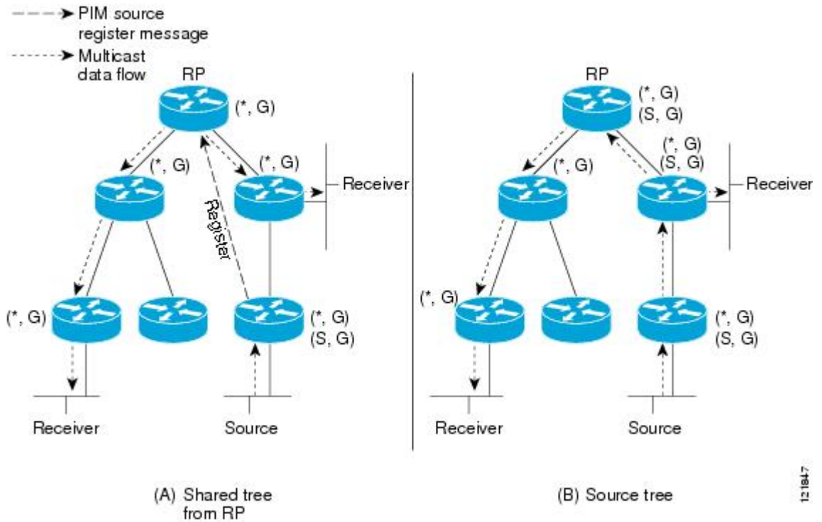
Figure 2: Unidirectional Shared Tree and Source Tree
