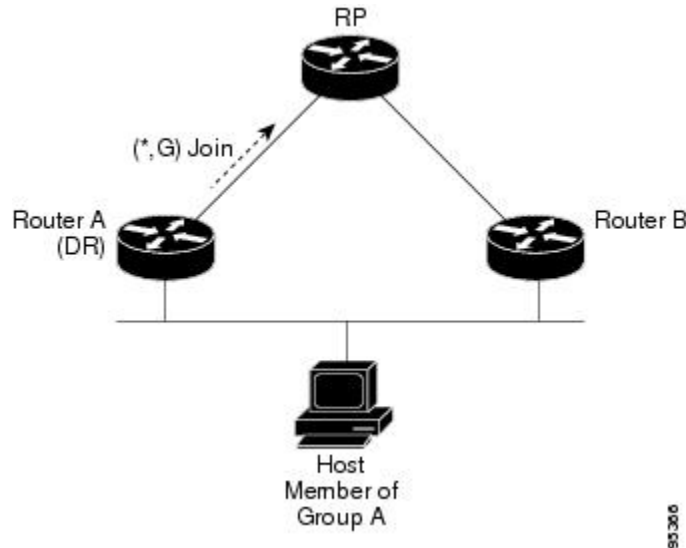
Figure 15: Designated Router Election on a Multiaccess Segment
