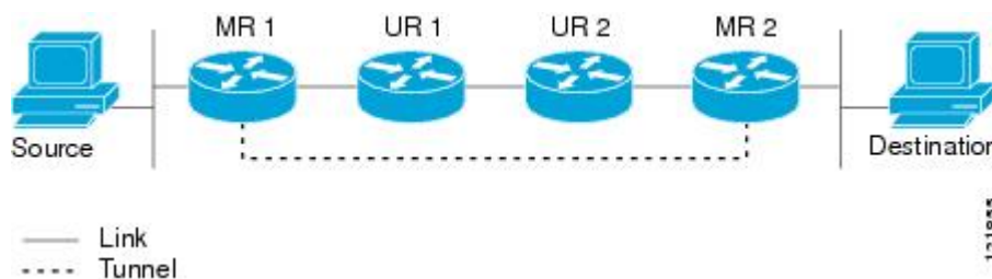
Figure 13: Tunnel for Multicast Packets
