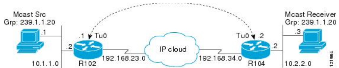
Figure 14: Tunnel Connecting Non-IP Multicast Areas
