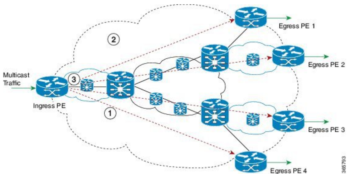
Figure 1: PE-PE Ingress Replication Topology
