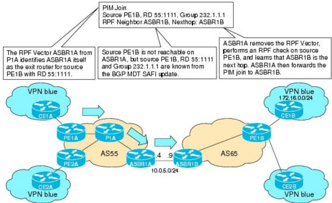
Figure 9 SSM Default MDT PIM Join from ASBR1A to ASBR1B
