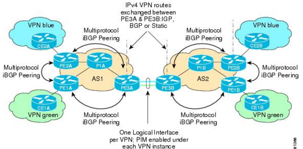
Figure 19 Topology for MVPN Inter-AS Support Option A Configuration Example
