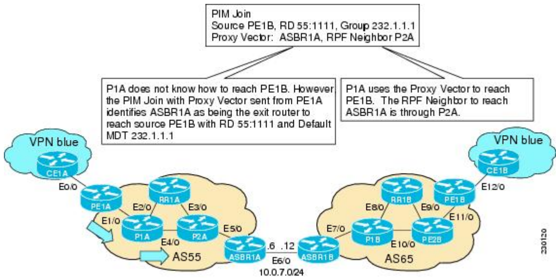
Figure 16 PIM SSM Join for Default MDT with Proxy Vector from P1A to P2A
