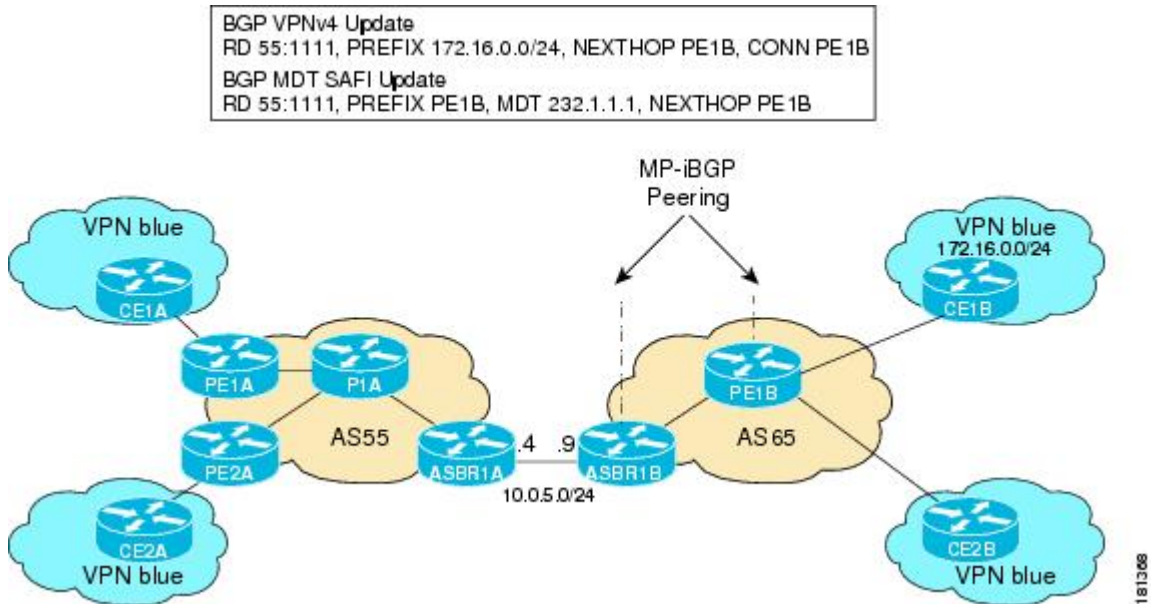
Figure 4 BGP Updates from PE1B to ASBR1B
