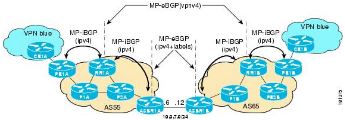
Figure 21 Topology for MVPN Inter-AS Support Option C Configuration Example
