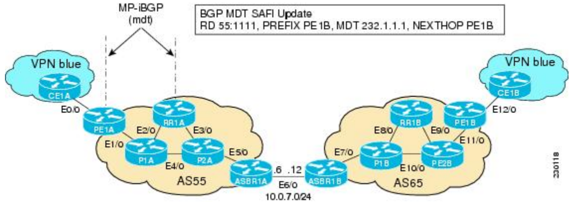
Figure 14 BGP MDT SAFI Update from RR1A to PE1A
