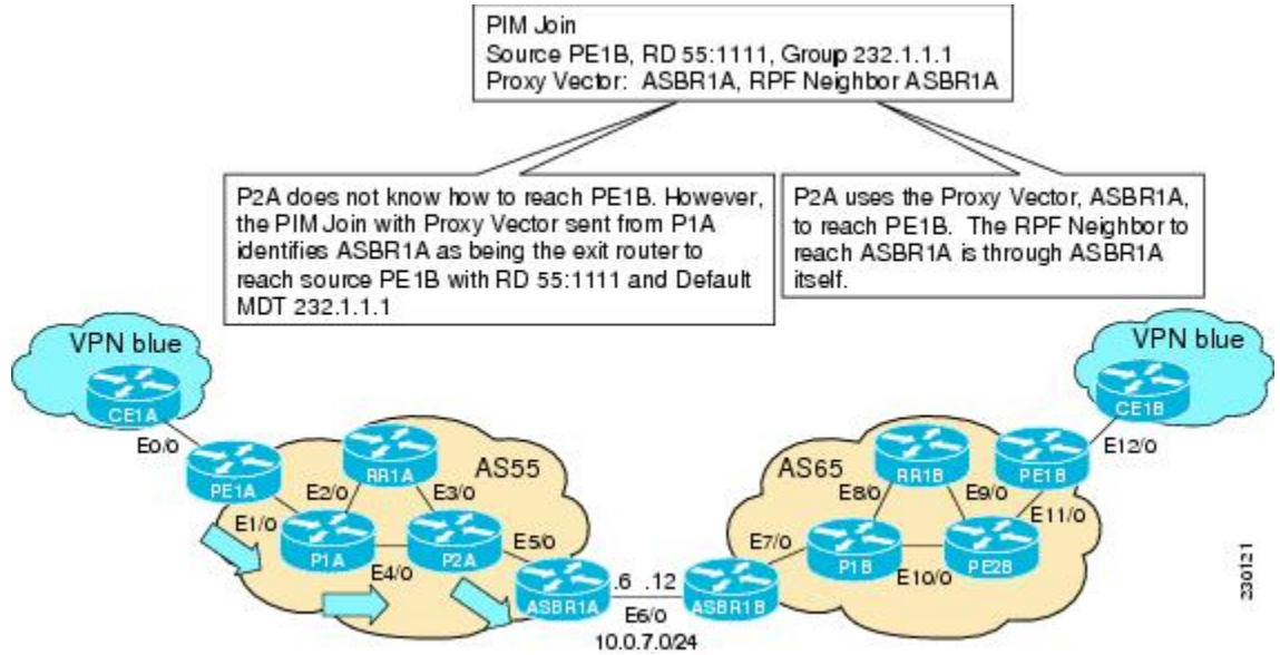
Figure 17 PIM SSM Join for Default MDT with Proxy Vector from P2A to ASBR1A
