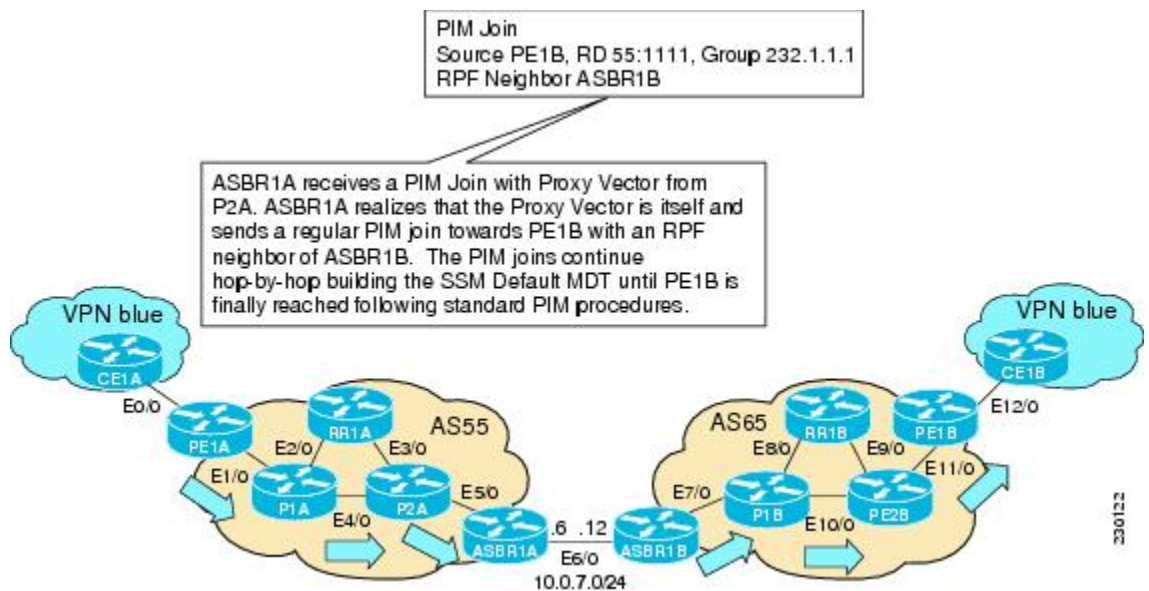
Figure 18 PIM SSM Join for Default MDT with Proxy Vector from ASBR1A to PE1B
