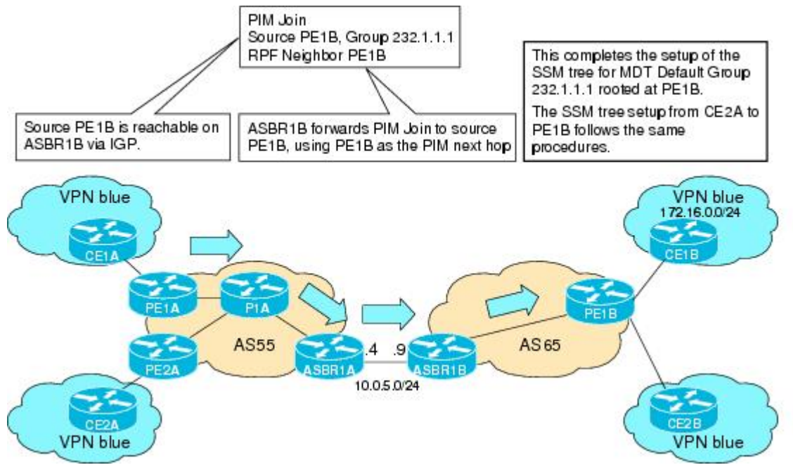
Figure 10 SSM Default MDT PIM Join from ASBR1B to PE1B
