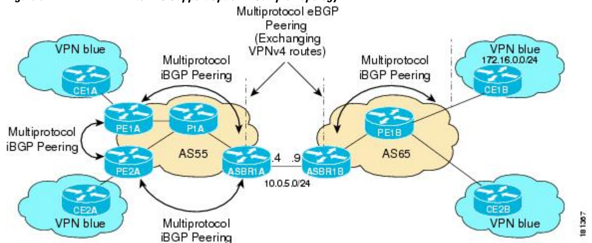
Figure 3 MVPN Inter-AS Support Option B Sample Topology
