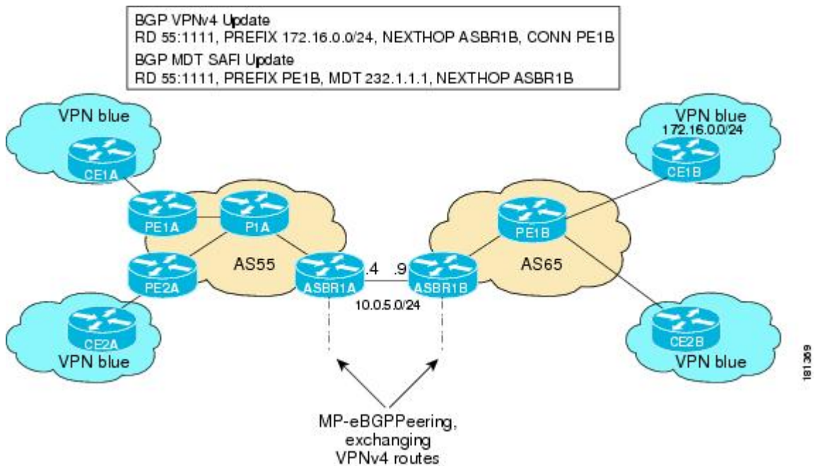
Figure 5 BGP Updates from ASBR1B to ASBR1A
