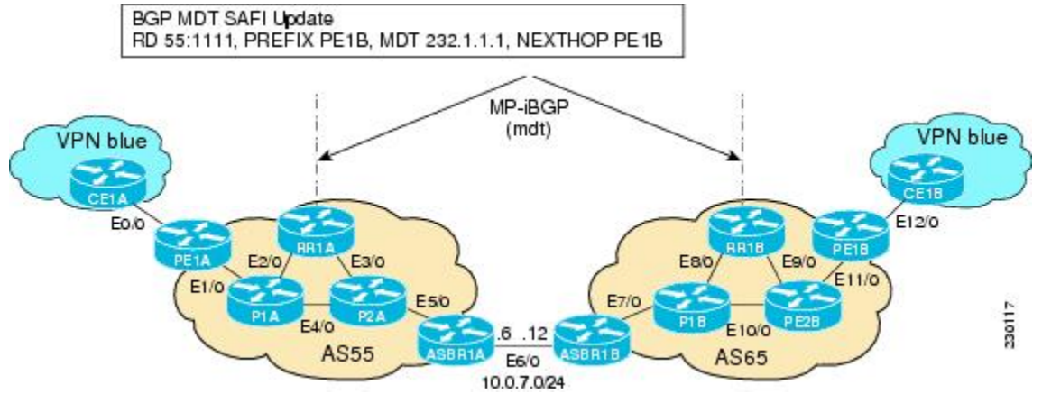
Figure 13 BGP MDT SAFI Update from RR1B to RR1A
