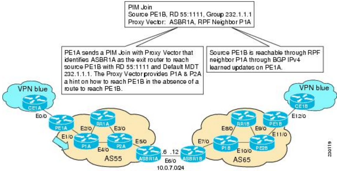
Figure 15 PIM SSM Join for Default MDT with Proxy Vector from PE1A to P1A
