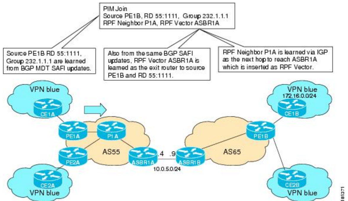
Figure 7 SSM Default PIM Join from PE1A to P1A
