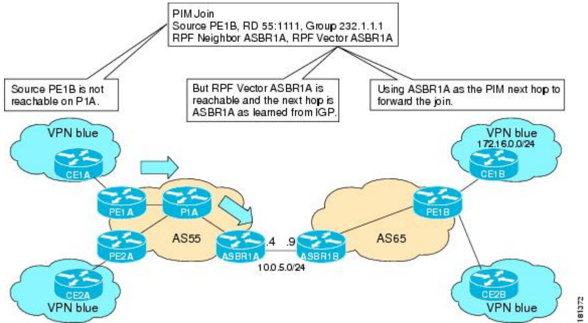
Figure 8 SSM Default MDT PIM Join from P1A to ASBR1A
