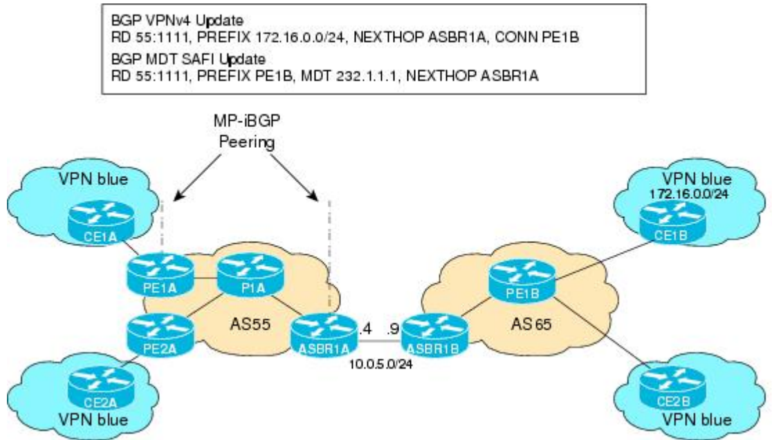
Figure 6 BGP Updates from ASBR1A to PE1A
