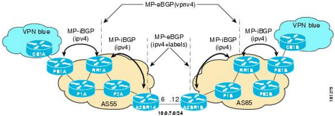
Figure 11 MVPN Inter-AS Support Option C Sample Topology
