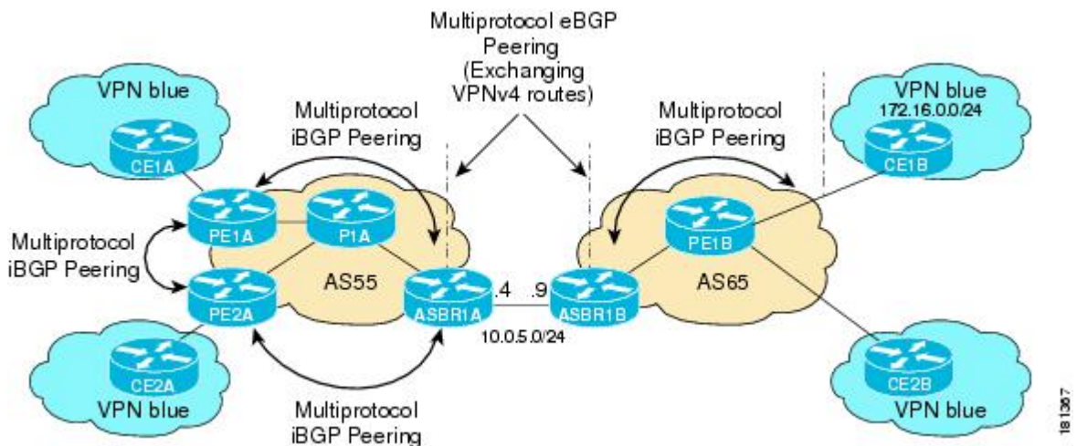
Figure 20 Topology for MVPN Inter-AS Support Option B Configuration Example
