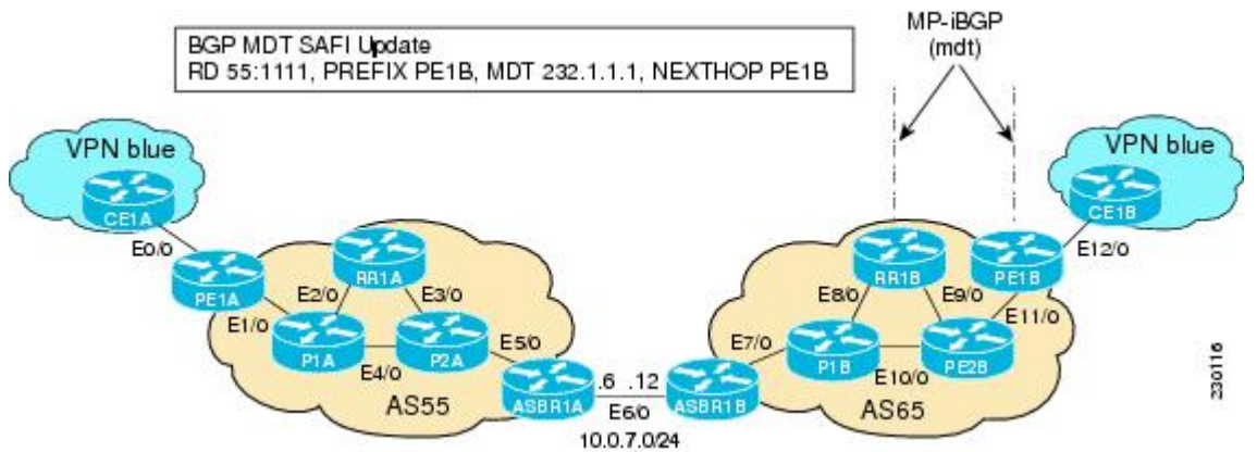
Figure 12 BGP MDT SAFI Update from PE1B to RR1B
