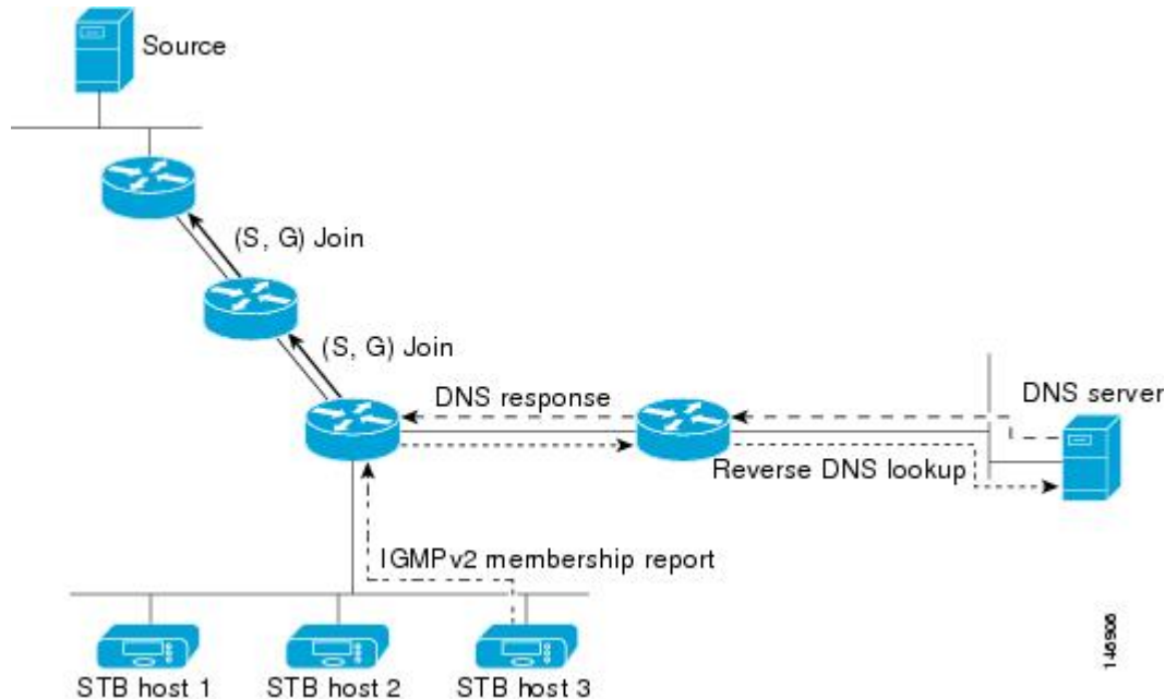
Figure 1 DNS-Based SSM-Mapping
