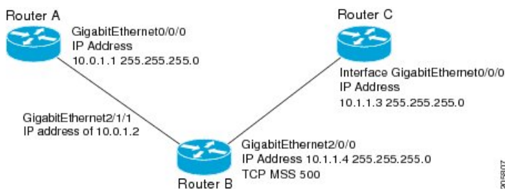
Figure 1: Example Topology for TCP MSS Adjustment
