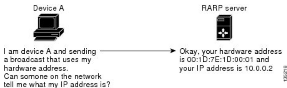
Figure 3: RARP Process
