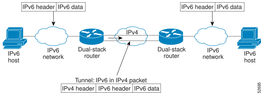
Figure 3 Overlay Tunnels
