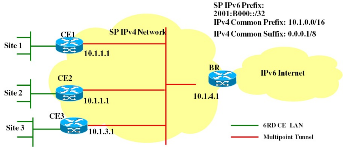
Figure 3: 6RD Prefix Delegation and Explanation
