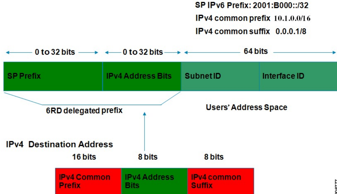
Figure 2: 6RD Prefix Delegation Explanation
