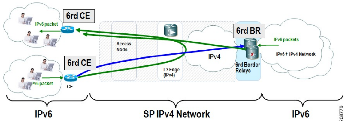
Figure 1: 6RD Deployment
