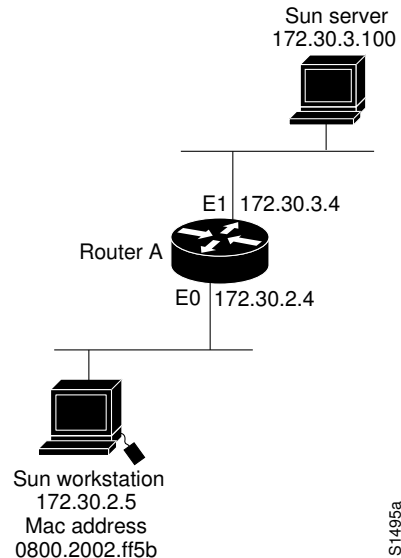
Figure 1 Configuring a Router As a RARP Server
