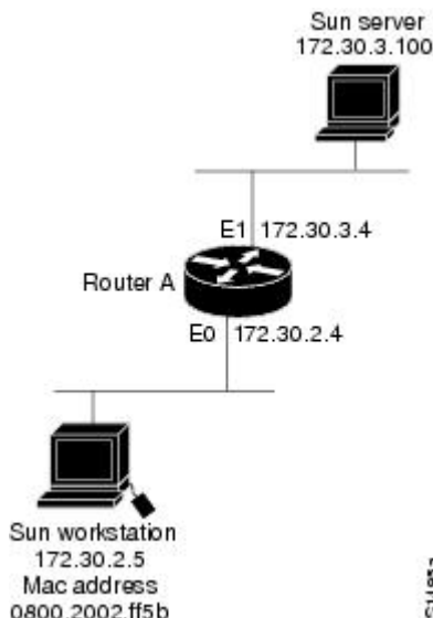
Figure 1: Configuring a Router As a RARP Server
