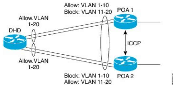
Figure 1: Active/Active Support
