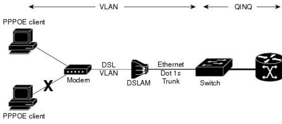
Figure 1: PPPoE over QinQ Session Limiting
