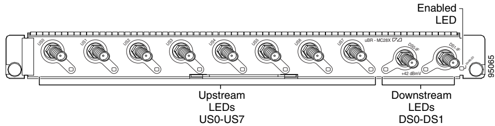
Figure 2 Cisco uBR-MC28X Cable Interface Line Card Front Panel
