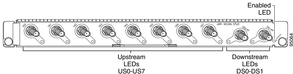
Figure 1 Cisco uBR-MC28U Cable Interface Line Card Front Panel
