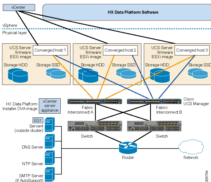
Figure 1: Cisco HyperFlex HX-Series System Component Details
